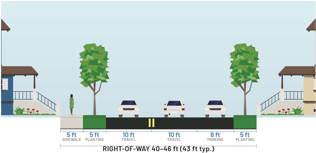
Representative section at typical right-of-way; widths are typical values from Table 3.1a. Cross-section illustration adapted from Streetmix (streetmix.net), © the Streetmix project, licensed CC BY-SA 4.0.
