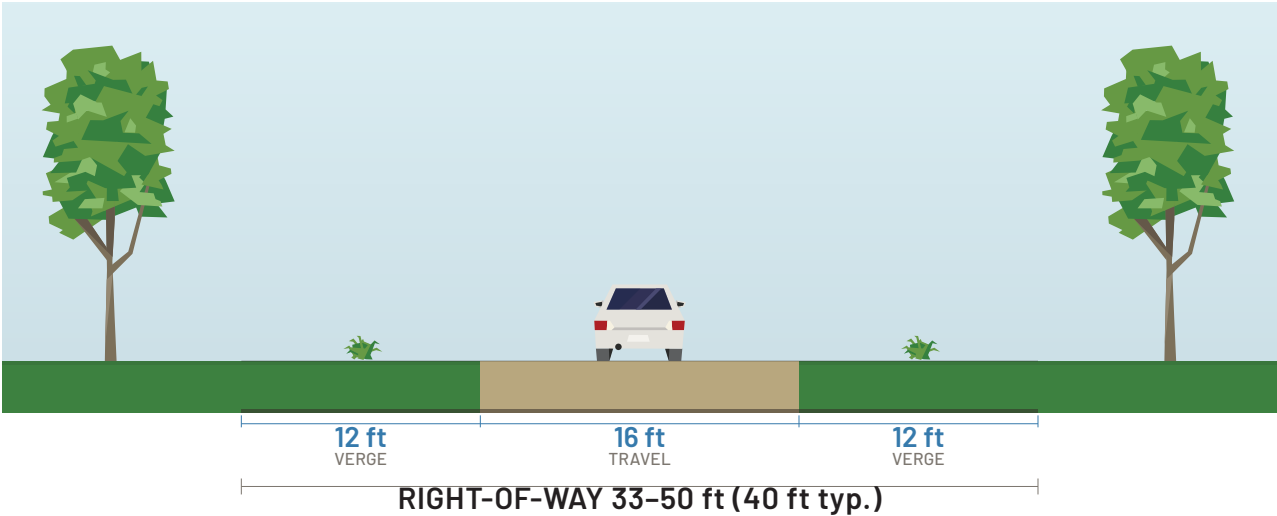
Representative section at typical right-of-way; widths are typical values from Table 3.1b. Cross-section illustration adapted from Streetmix (streetmix.net), © the Streetmix project, licensed CC BY-SA 4.0.
